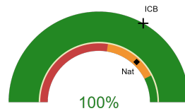
Estimated case ascertainment 01 April 2025 - 30 June 2025
